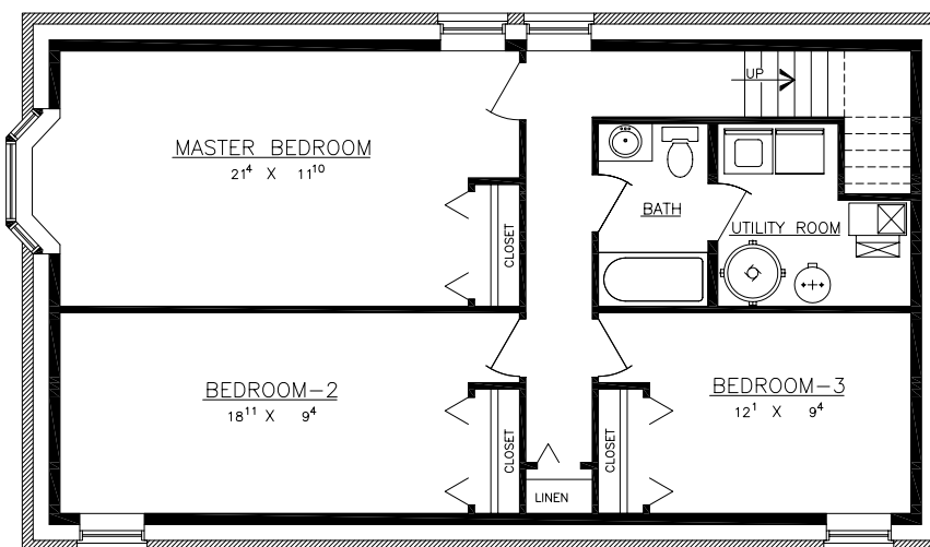
GROUND FLOOR AREA = 1008 S.F.
